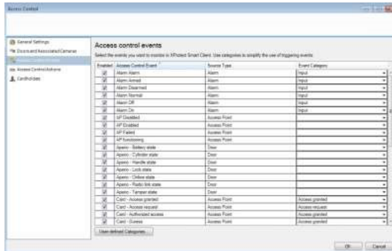
Figure 26: Configuration of the access control events and link between specific events from the SCNET4 system and generic access control events in the plugin.
