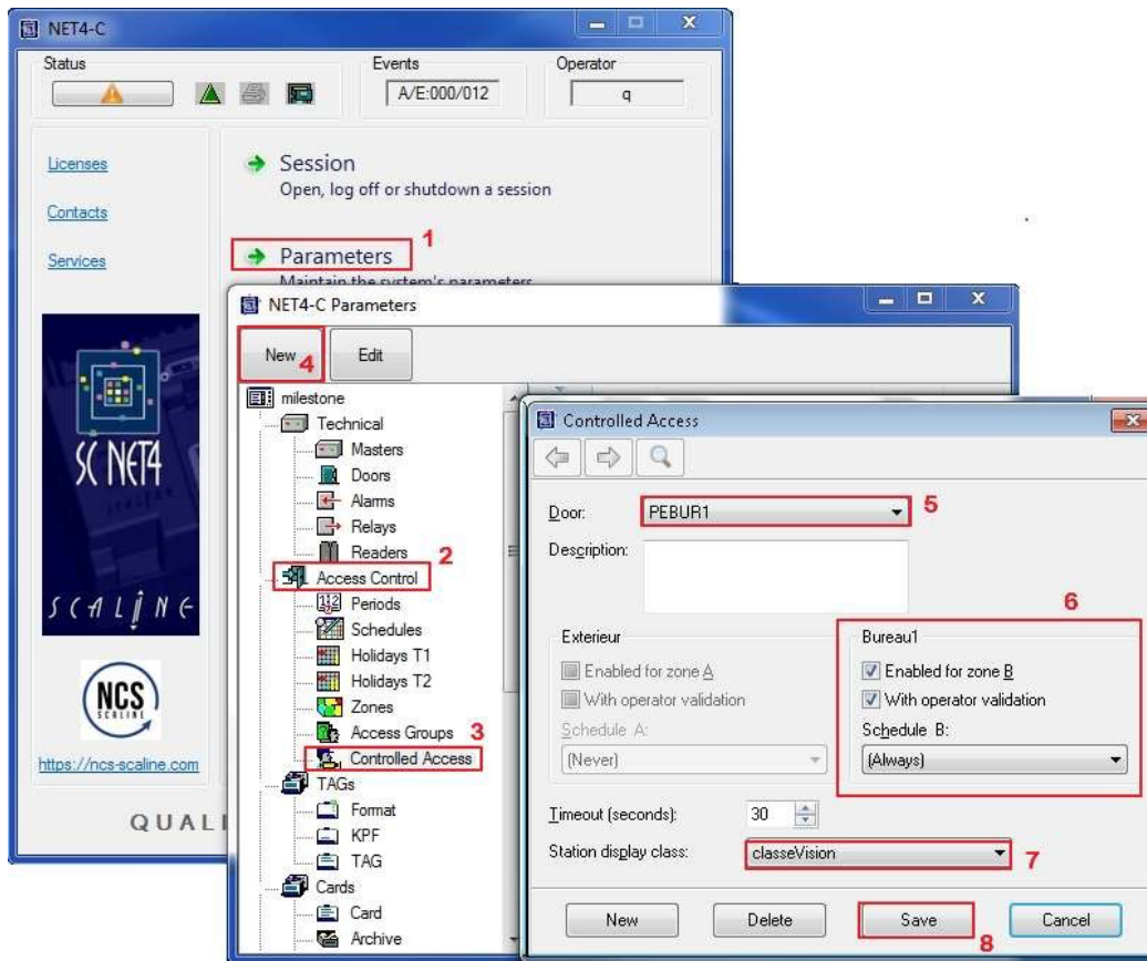
Figure 8: Controlled access setup to enable management from MOBOTIX HUB Desk Client HUB.
