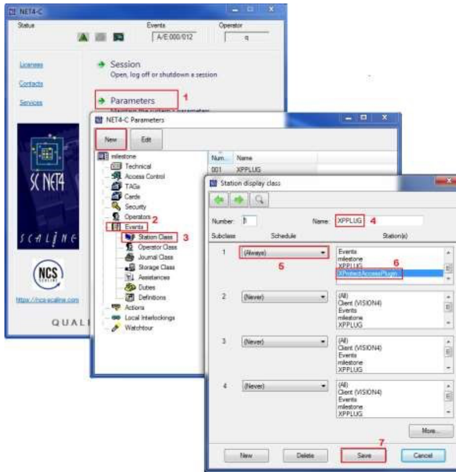
Figure 7: Station display class required in order to setup the controlled access with the XPPLUG plugin.
