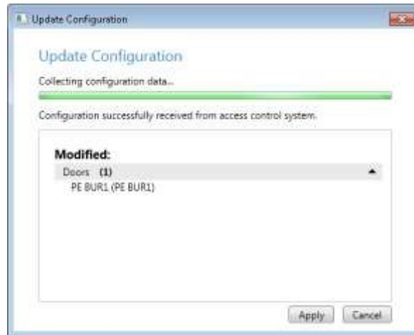
Figure 24: Illustration of the detection of an additional doors during the synchronization between the SCNET4 system and the XPPLUG MOBOTIX HUB Access plugin.
