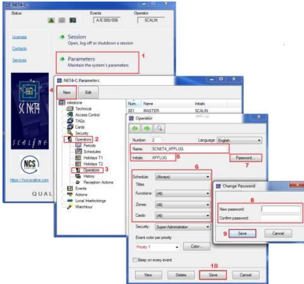
Figure 4: Configuration of a dedicated operator in the NET4-C interface.
