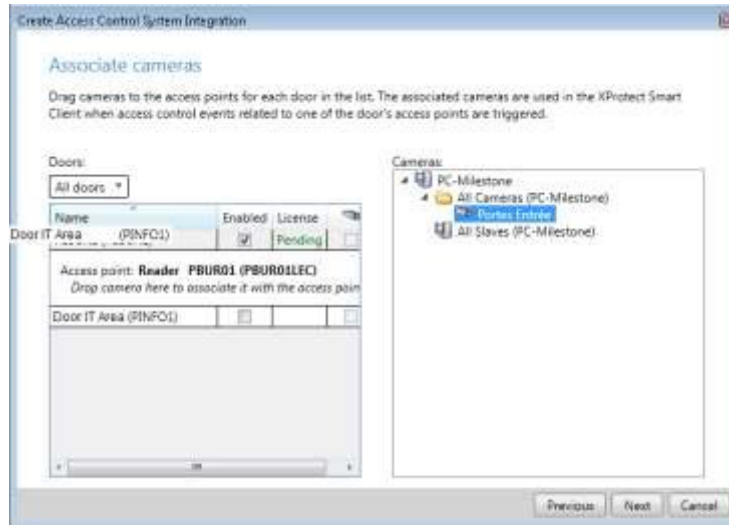
Figure 21: Association of cameras with doors/ access points of the MOBOTIX HUB Access Control plugin.
