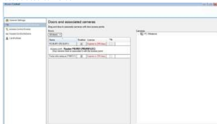
Figure 25: Configuration of the door/access-point – camera association
