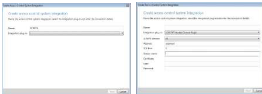
Figure 19: Selection of the target plugin and configuration of its generic parameters.
