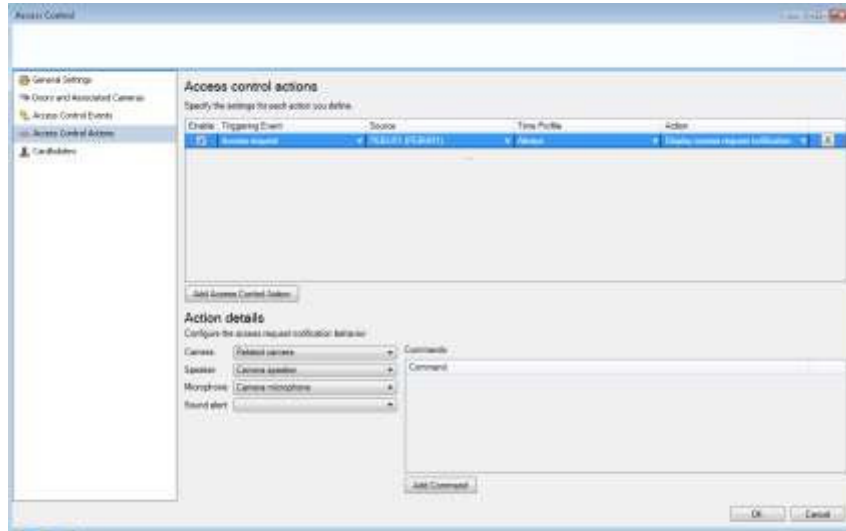
Figure 27: Configuration of access control functions in MOBOTIX HUB
